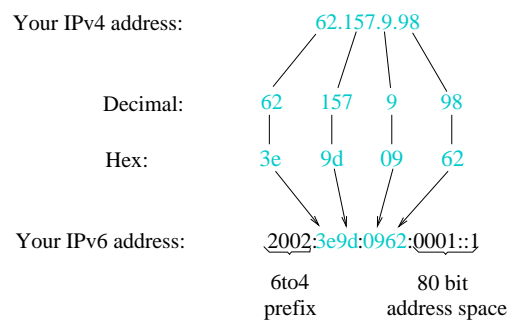
Figure 8-8. 6to4 derives a IPv6 from an IPv4 address
