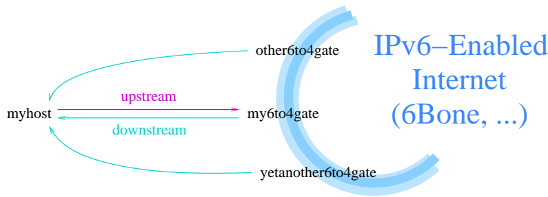
Figure 8-9. Request and reply can be routed via different gateways in 6to4
