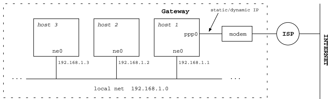
Figure 8-6. Network with gateway
