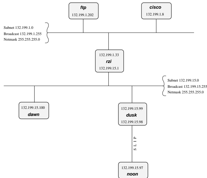
Figure 8-1. Our demo-network
