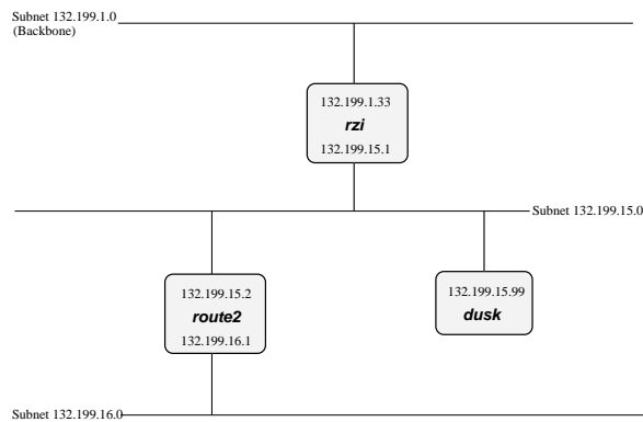
Figure 8-2. Attaching one subnet to another one
